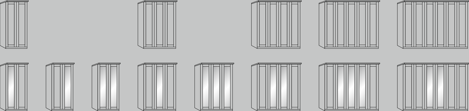
Hinged-door wardrobes doors in carcase colour with or without mirrored glass, W 100 – 300 cm, H 220 cm, D 58 cm
